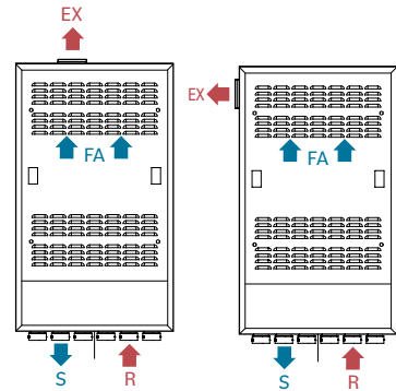
Position des Abluftkanals Exhaust air duct position
