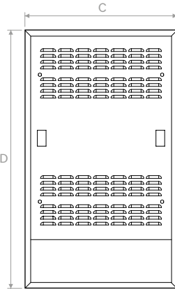
Frontansicht Front view
