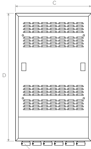
Ștuț racord pentru tub striat Ø75/90 Plug spigots for corrugated hose Ø75/90
